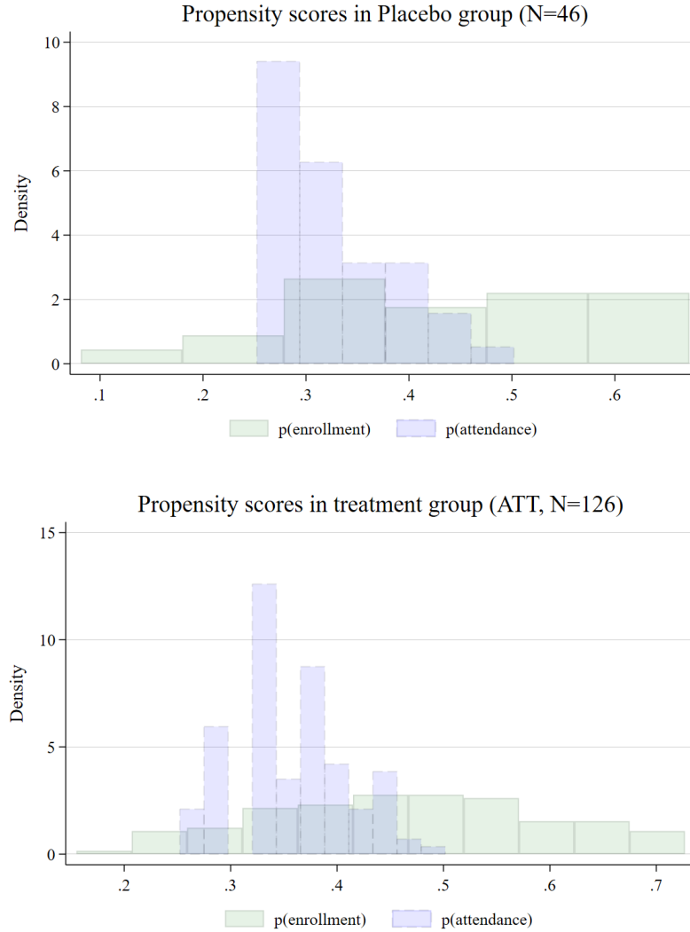
Figure A6: Propensity scores in Placebo and treatment groups
